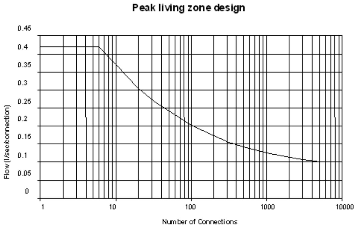
Figure 1 - Peak living zone on demand supply design flow rates
