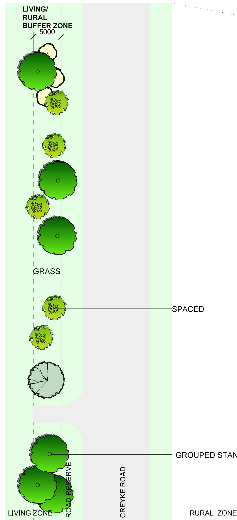
PLAN SECTION - LIVING/ RURAL BUFFER ZONE SCALE 1:400 @A3
