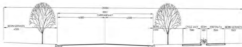
CONCEPT ROAD SECTION (WITH CYCLE WAY)
