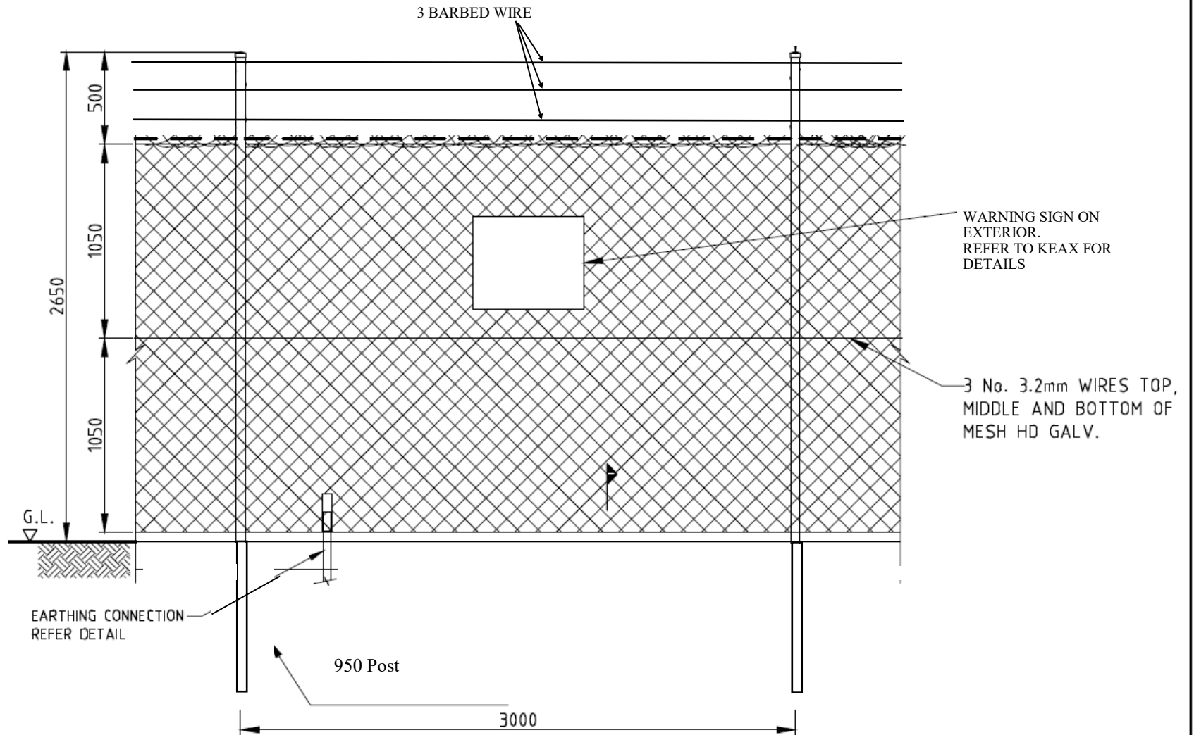
TYPICAL FENCE DETAIL
