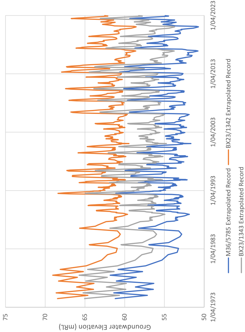
Figure 6: Extrapolated records (groundwater elevation) based on M36/0217
