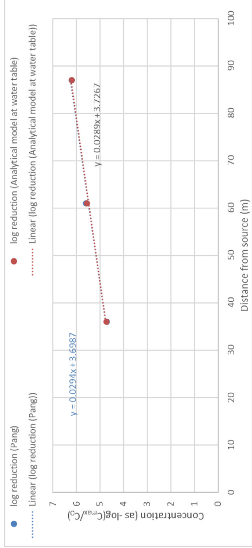
Figure 3: Modelled and observed (Pang, 1998) log reduction with distance from a source
