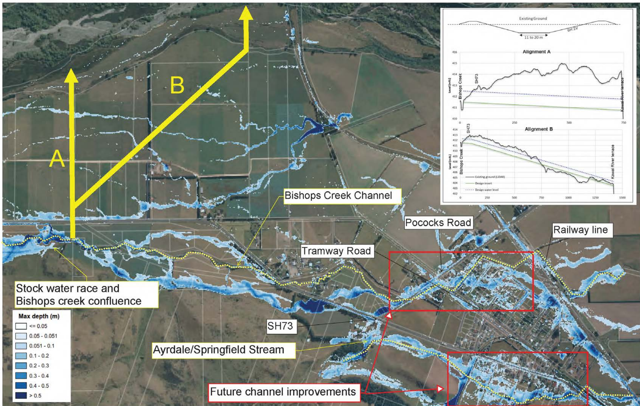
Flow diversion concept routes (Flood map: 2% AEP flood event 6-hour duration with 20 \text{ m}^3/\text{s} diversion)
