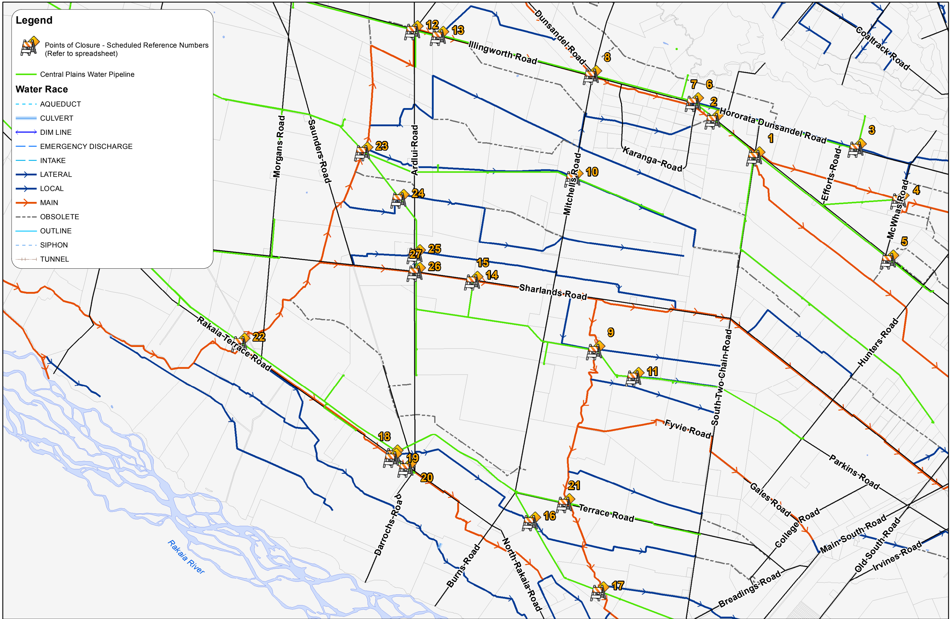
Water Race Closures for Pipeline Construction
